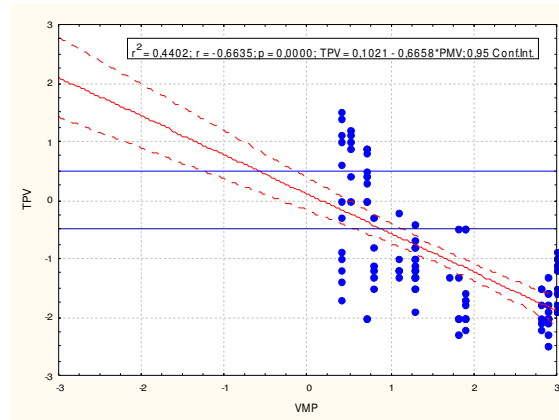
Figure 4 – Correlation between the TPV and the PMV in the naturally ventilated buildings
